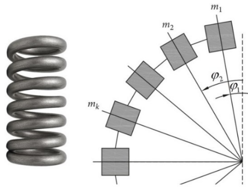
Figure 7: Discretized spring
